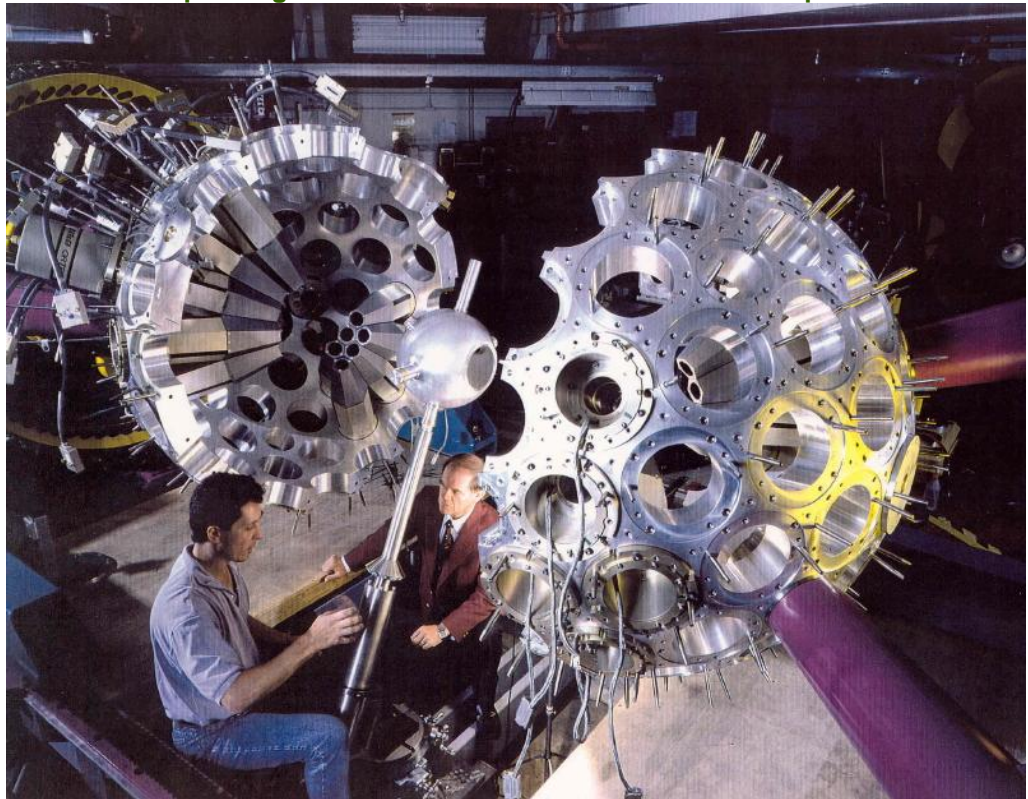
Complex High Vacuum Chambers and Machined Components
