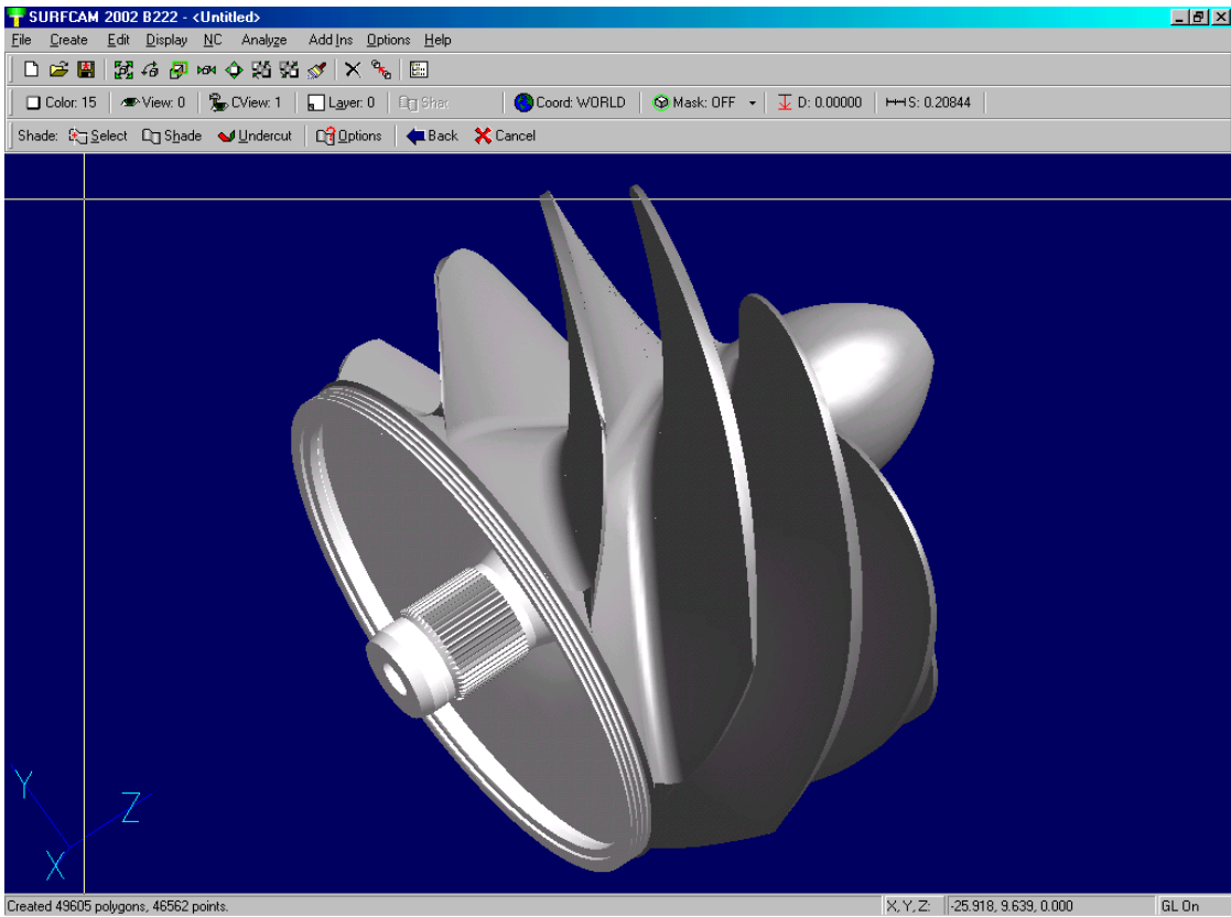
26 Inch Diameter Titanium Impeller Machined From 3D CAD Database
